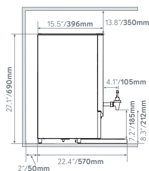
ECOBOILER T30 1000663
