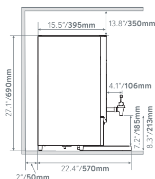
ECOBOILER T20 1000662
