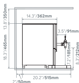
ECOBOILER T20 1000662
