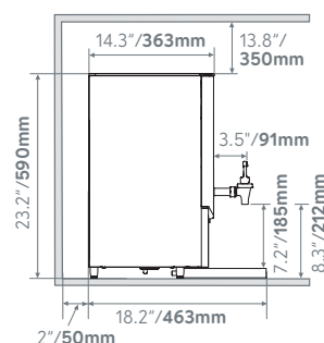
ECOBOILER T30 1000663
